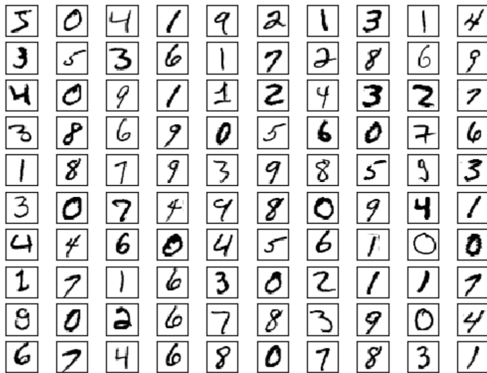
Figure 19-1. MNIST images
